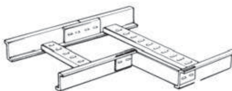
Offset Reduction Splice Set
