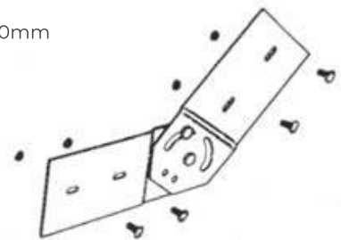
Adjustable Splice
