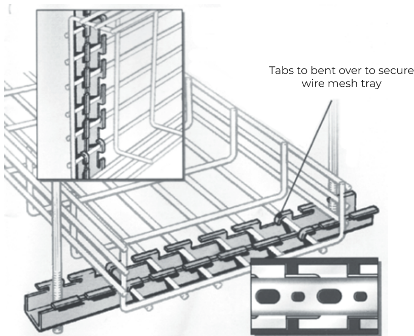
Clip-on Support Channel
