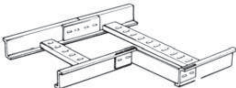
Offset Reduction Splice Set
